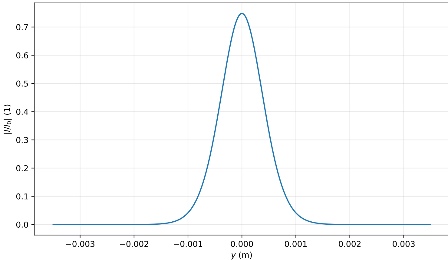
Intensity profile I(x=0, y, z=1.672)/I_0 , P_{in}=0.3P_{cr} , artificial time
